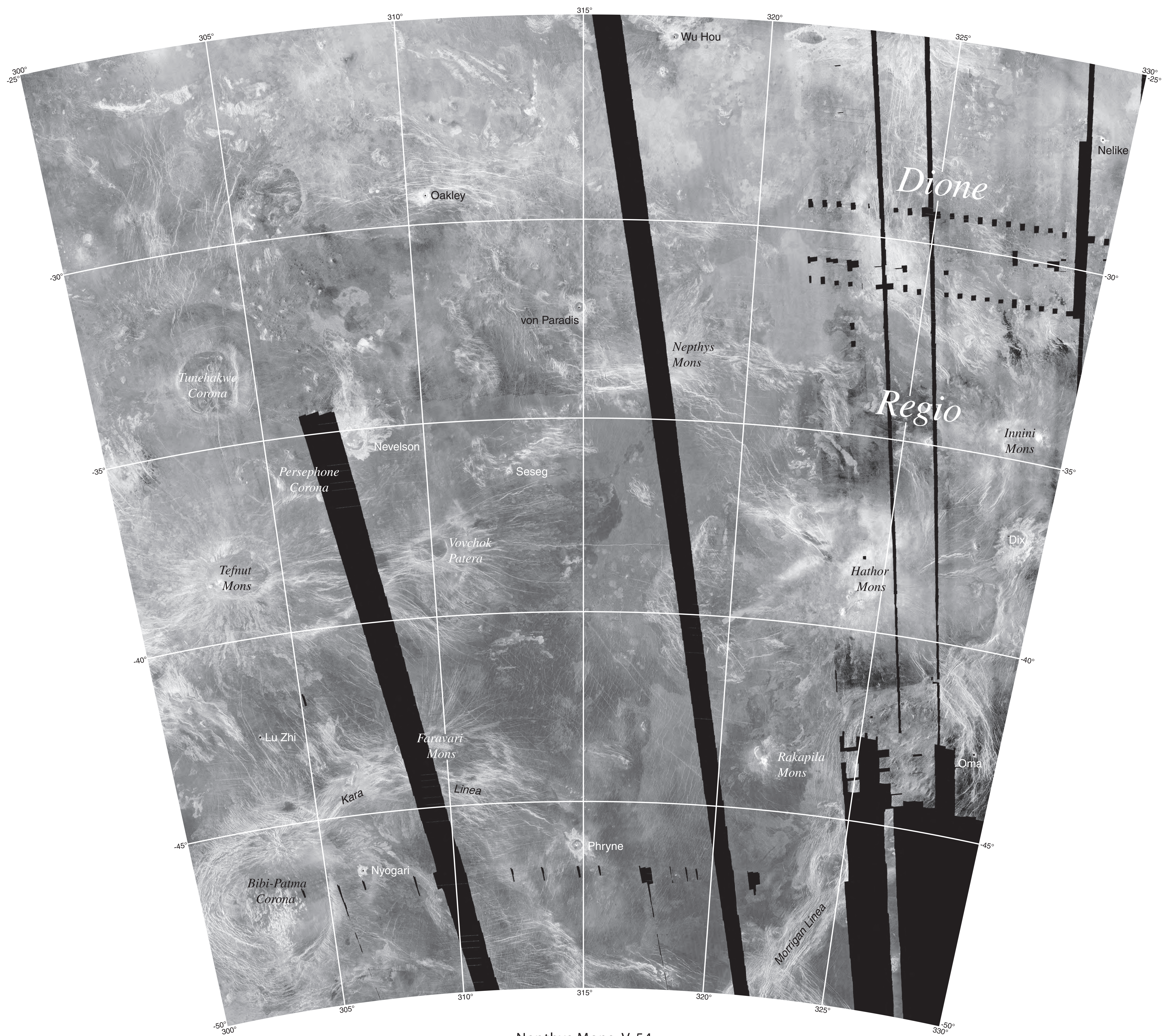
Nephys Mons, V-54 Lambert projection
