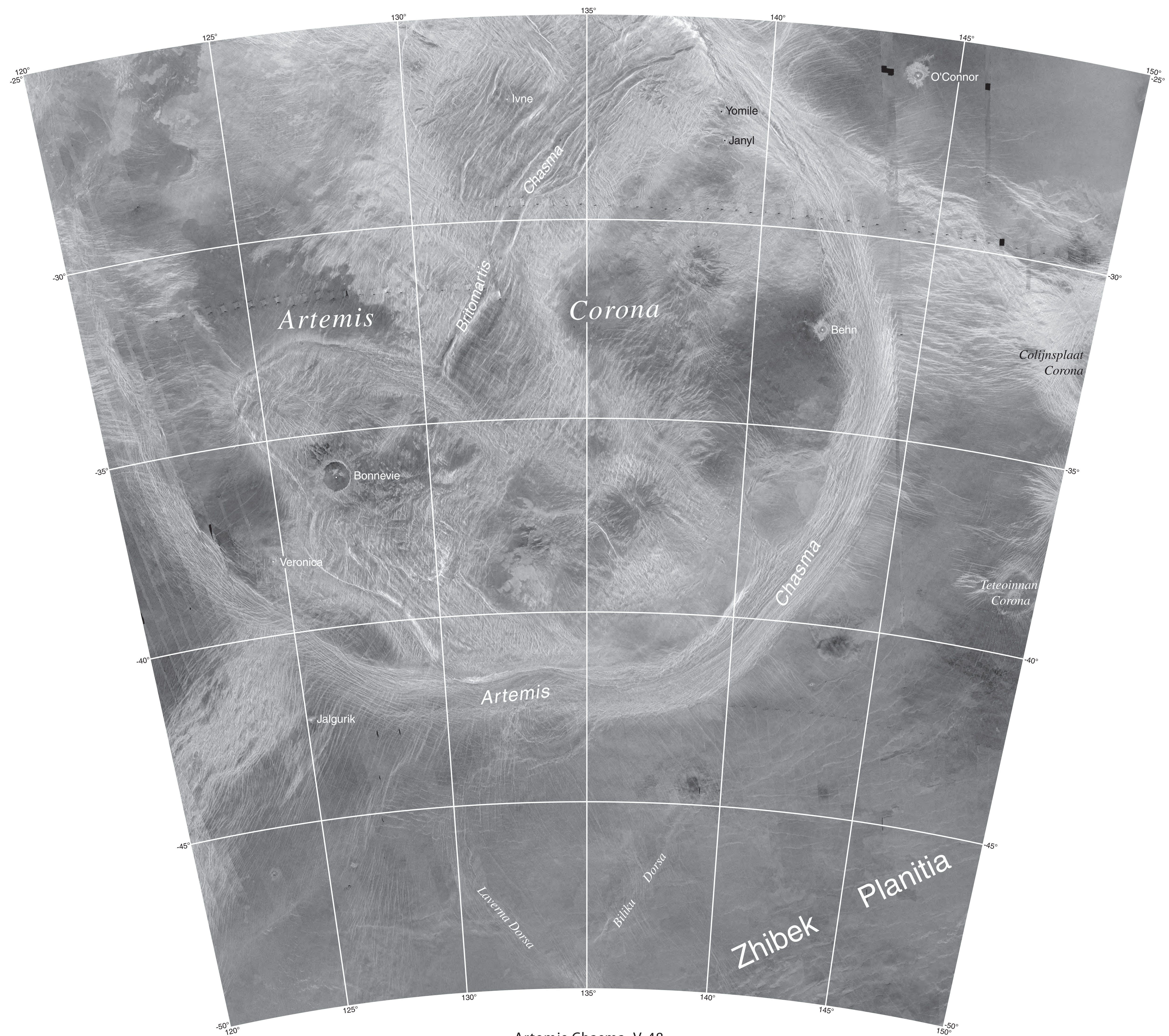
Artemis Chasma, V-48 Lambert projection
