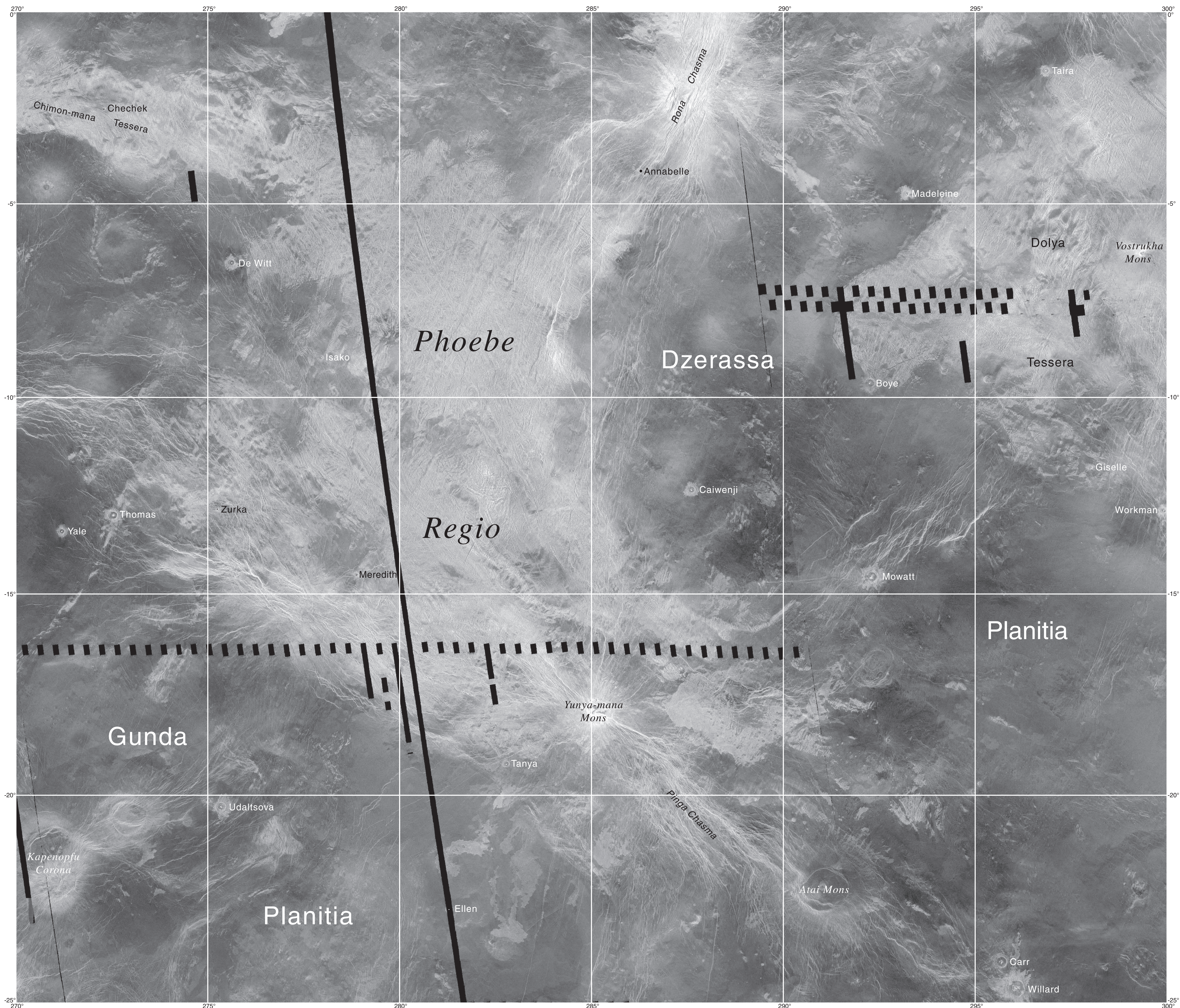
Phoebe Regio, V-41 Mercator projection Date of Last Nomenclature Update: August 18, 2017
