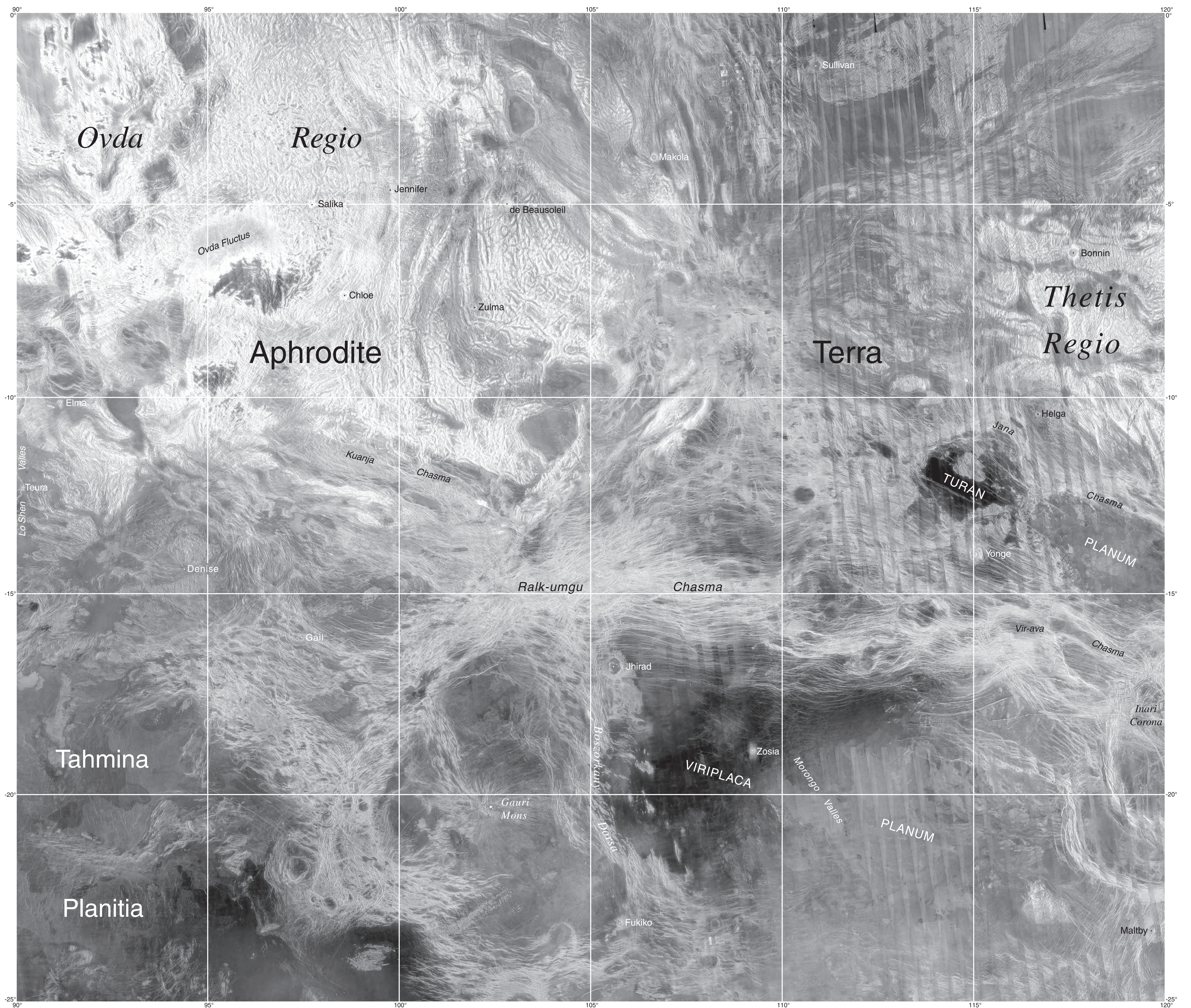
Ovda Regio, V-35 Mercator projection
