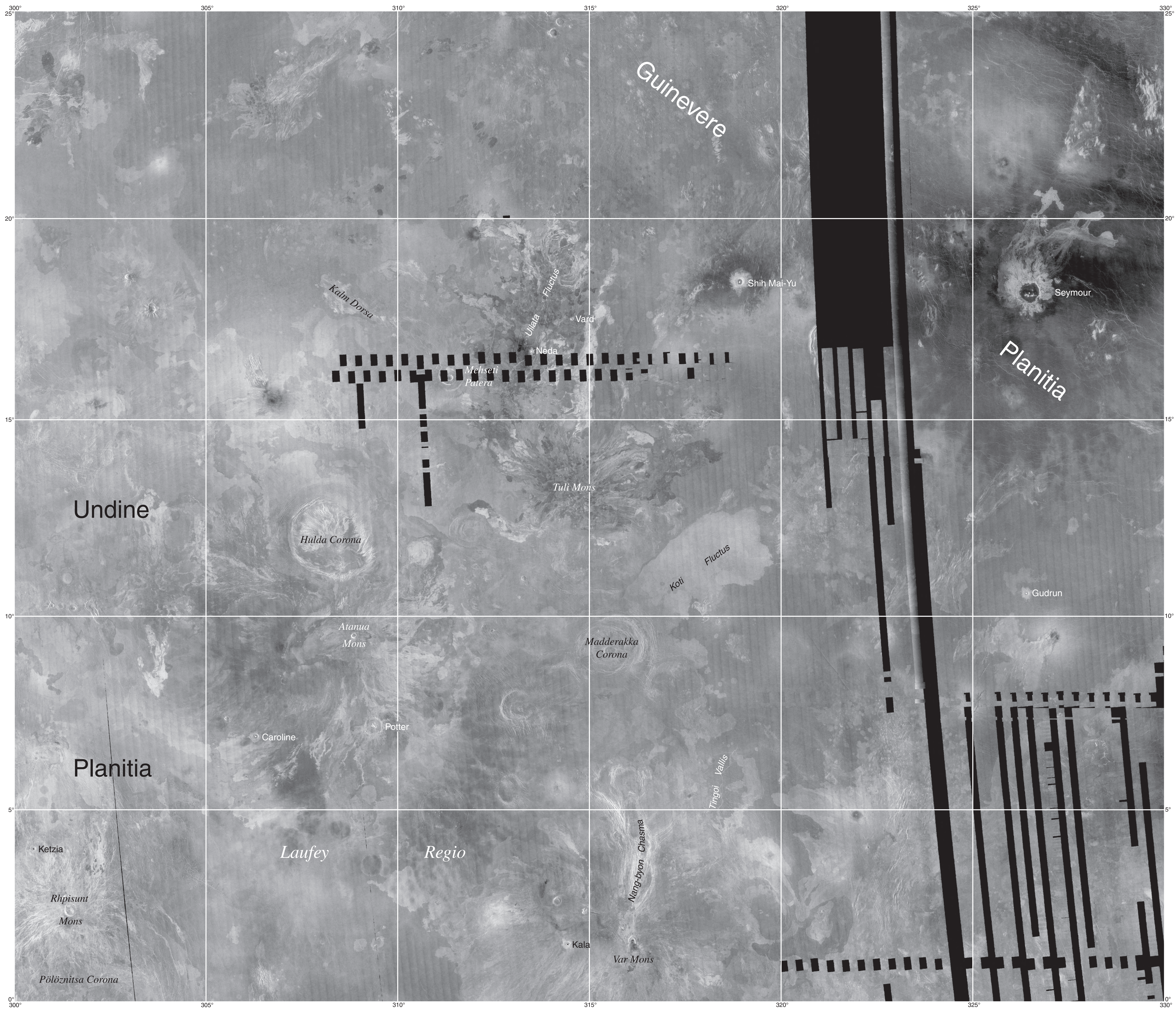
Guinevere Planitia, V-30 Mercator projection
