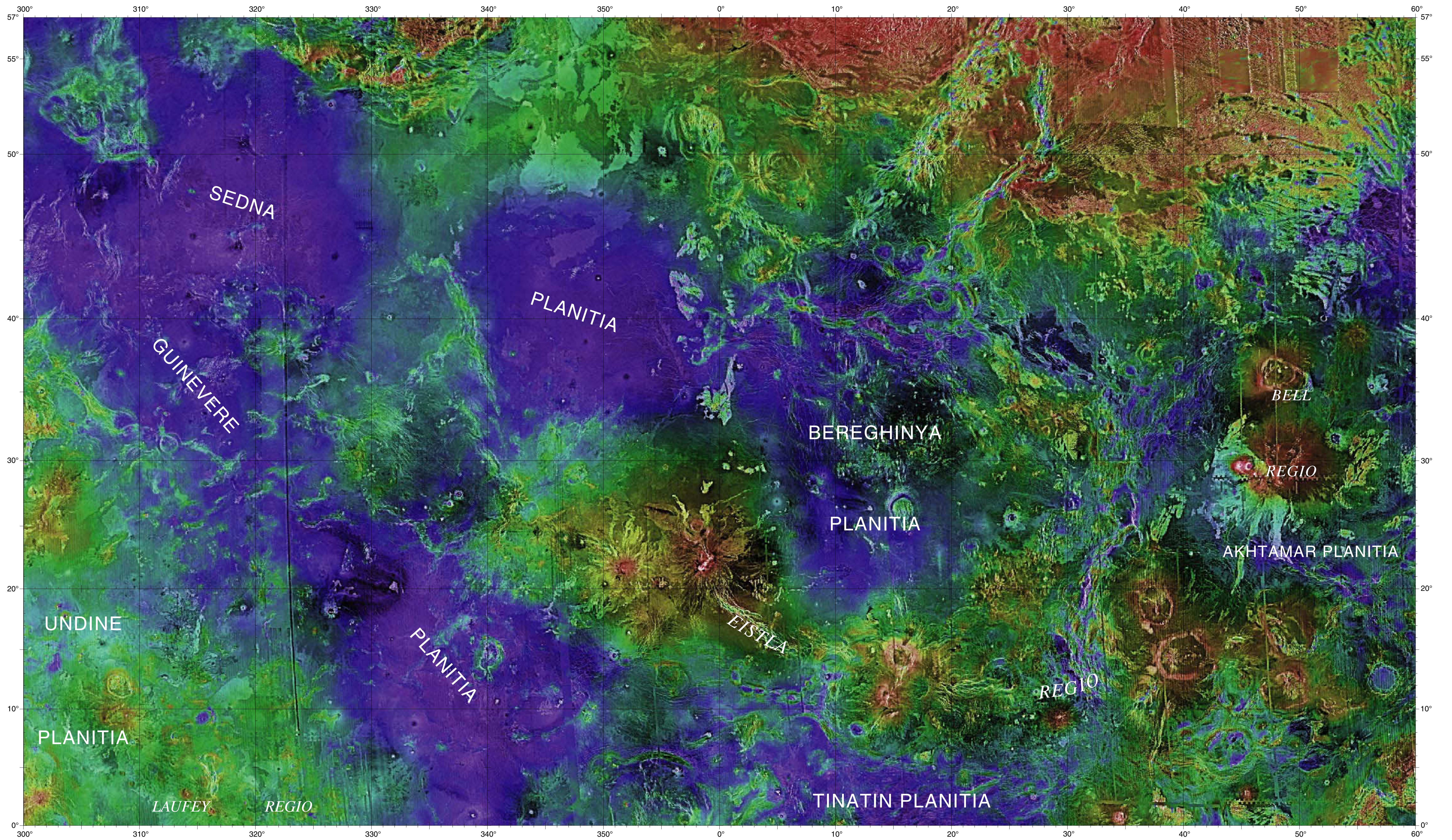
ALTIMETRIC RADAR IMAGE MAP OF THE SEDNA PLANITIA REGION OF VENUS
