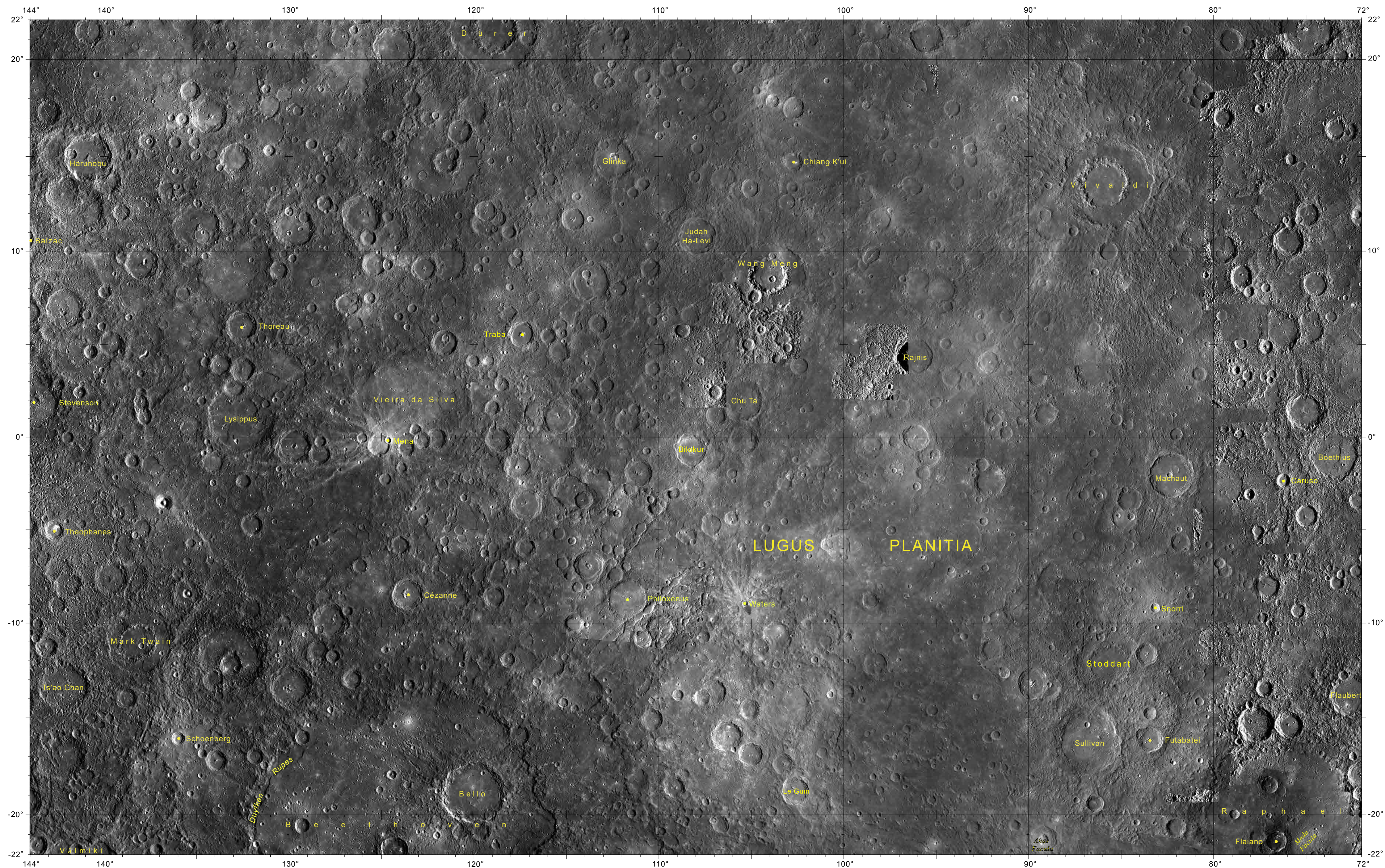
Map of the H-7 (Beethoven) Quadrangle of Mercury
