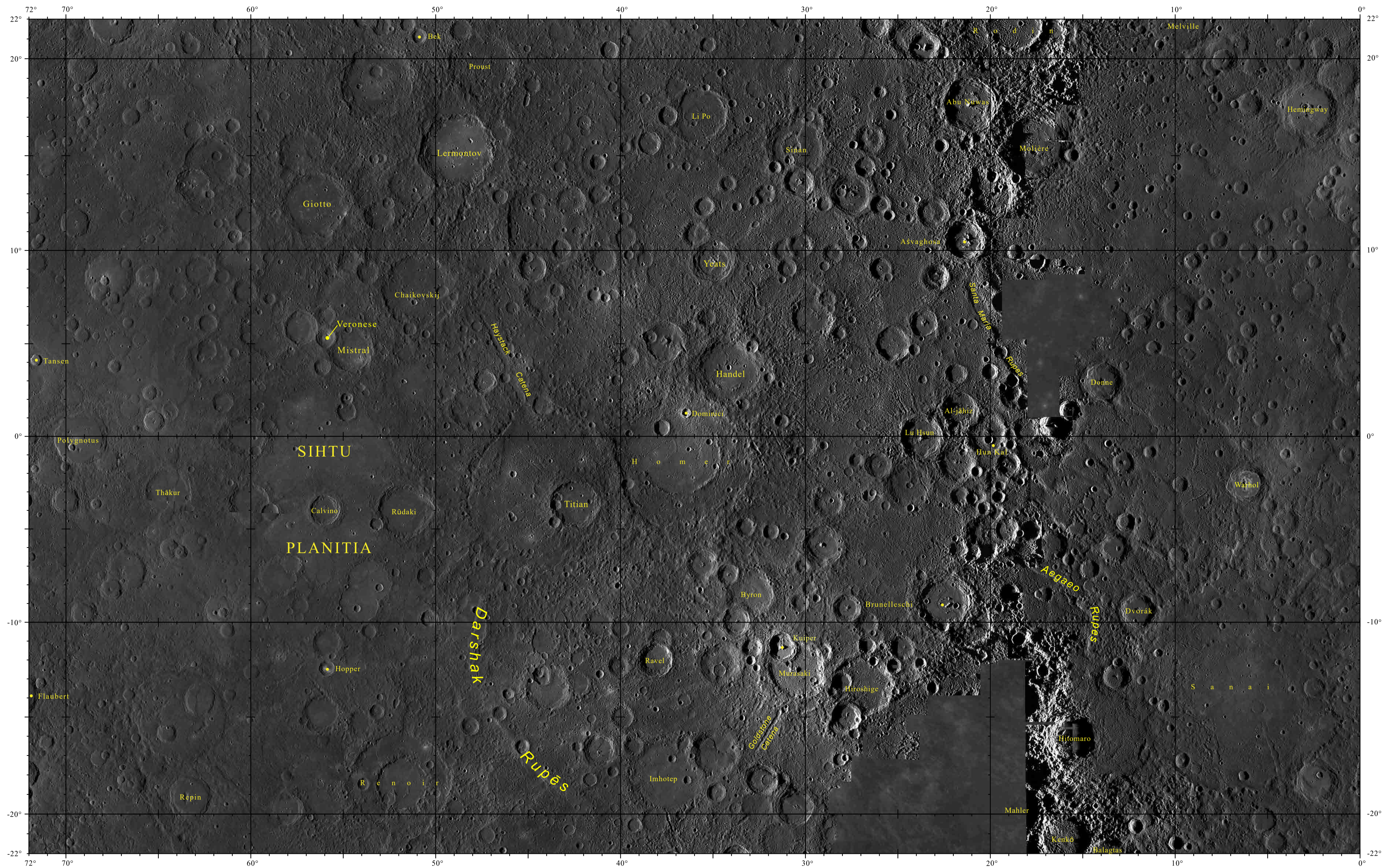
Map of the H-6 (Kuiper) Quadrangle of Mercury
