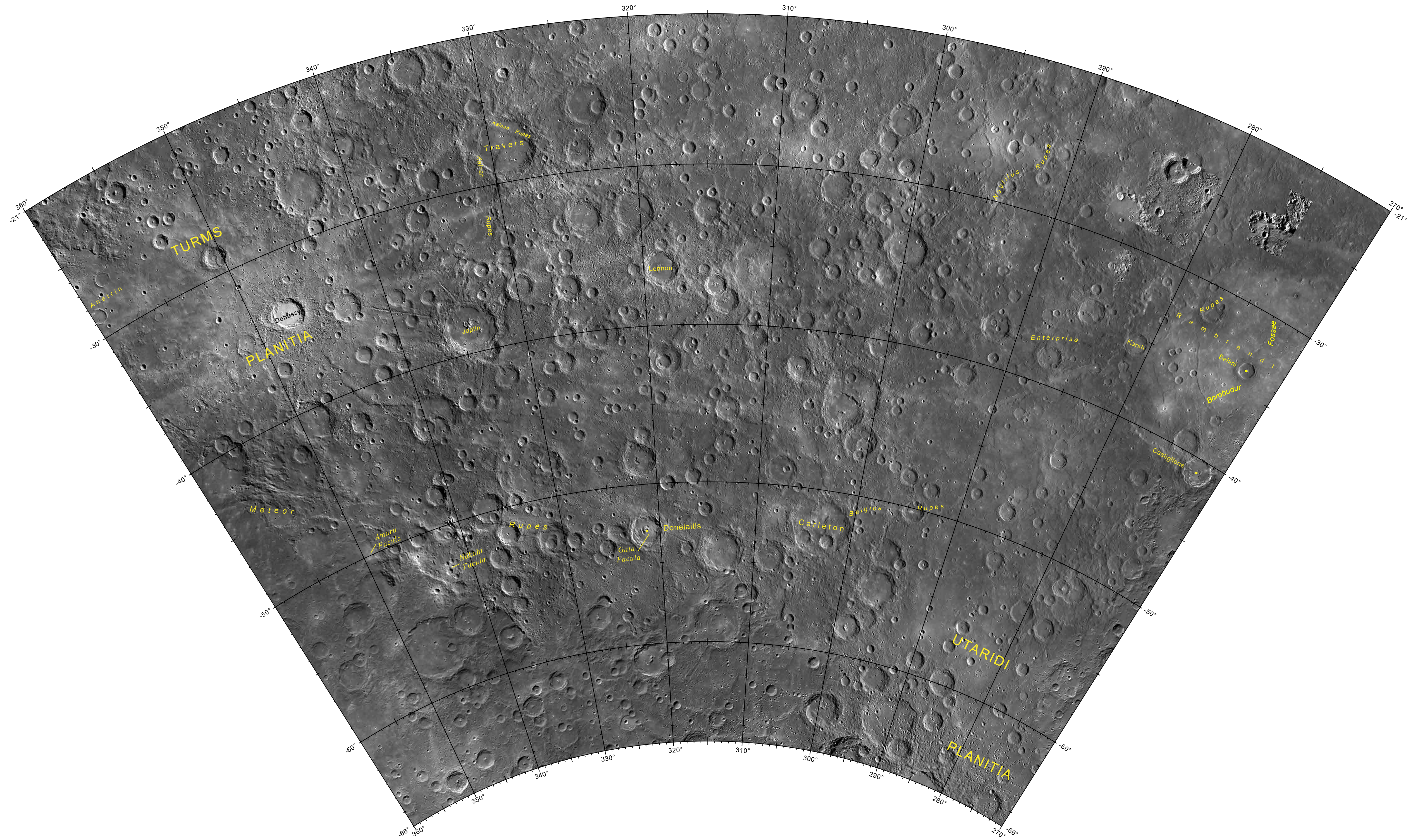
Map of the H-14 (Debussy) Quadrangle of Mercury
