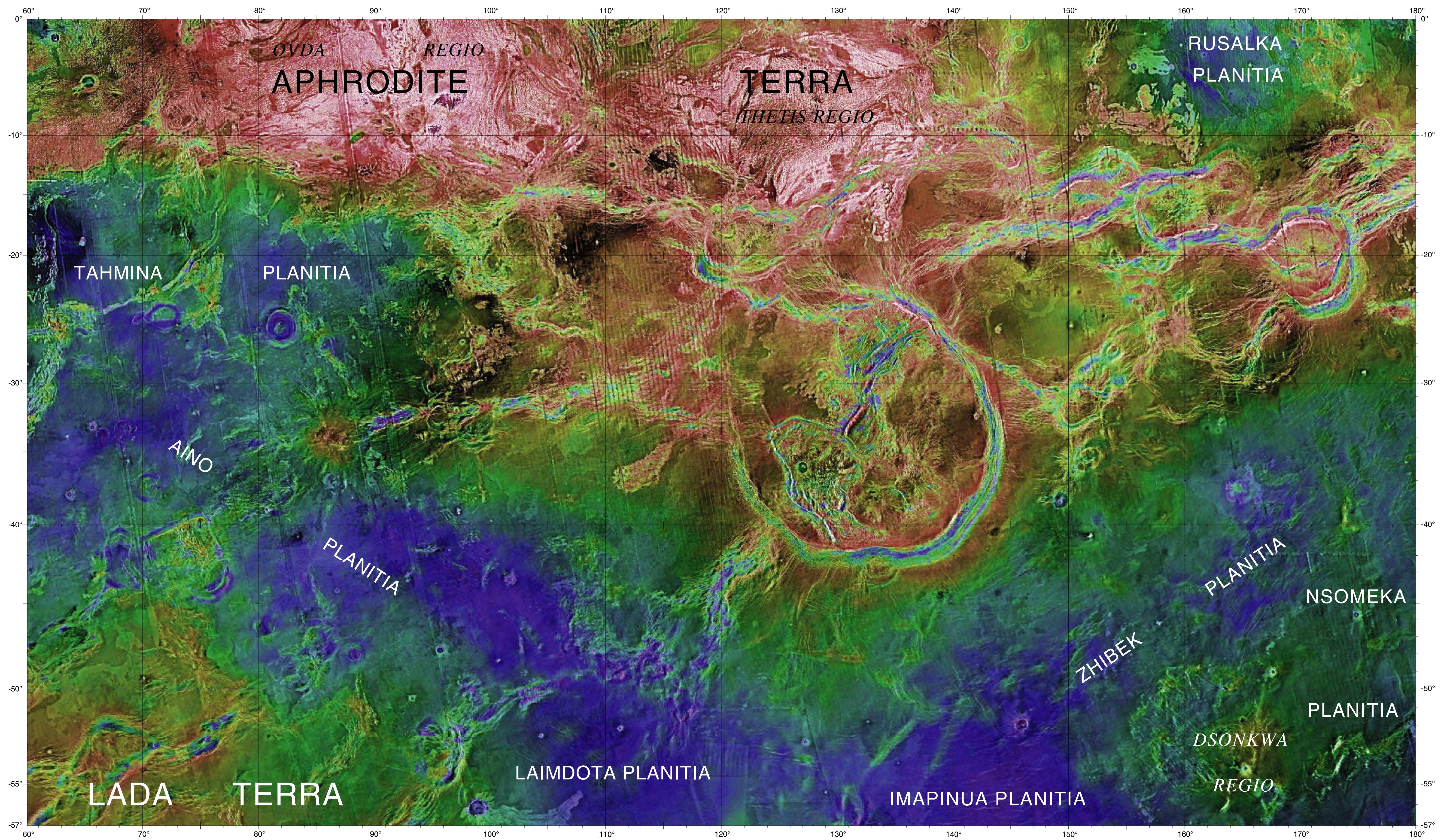
ALTIMETRIC RADAR IMAGE MAP OF THE APHRODITE TERRA REGION OF VENUS
